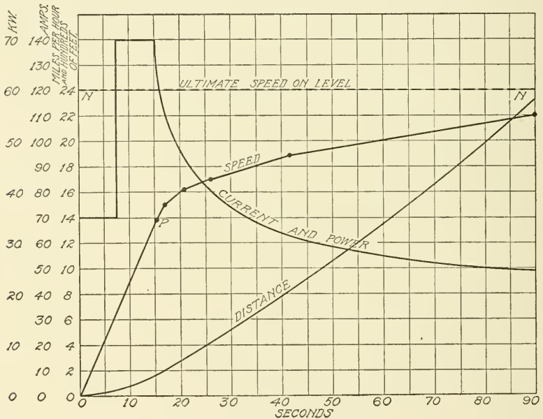
Fig. 131. Speed Curves
